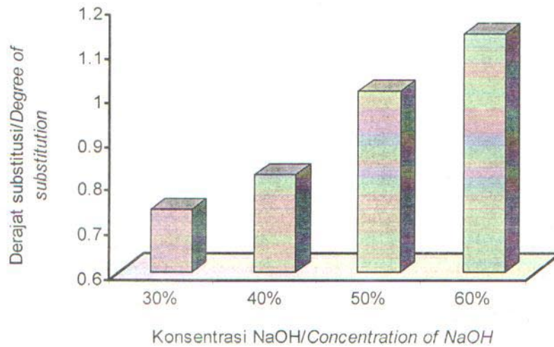
Gambar 4. Derajat substitusi Na-CMC. Figure 4. Degree of substitution of Na-CMC.
